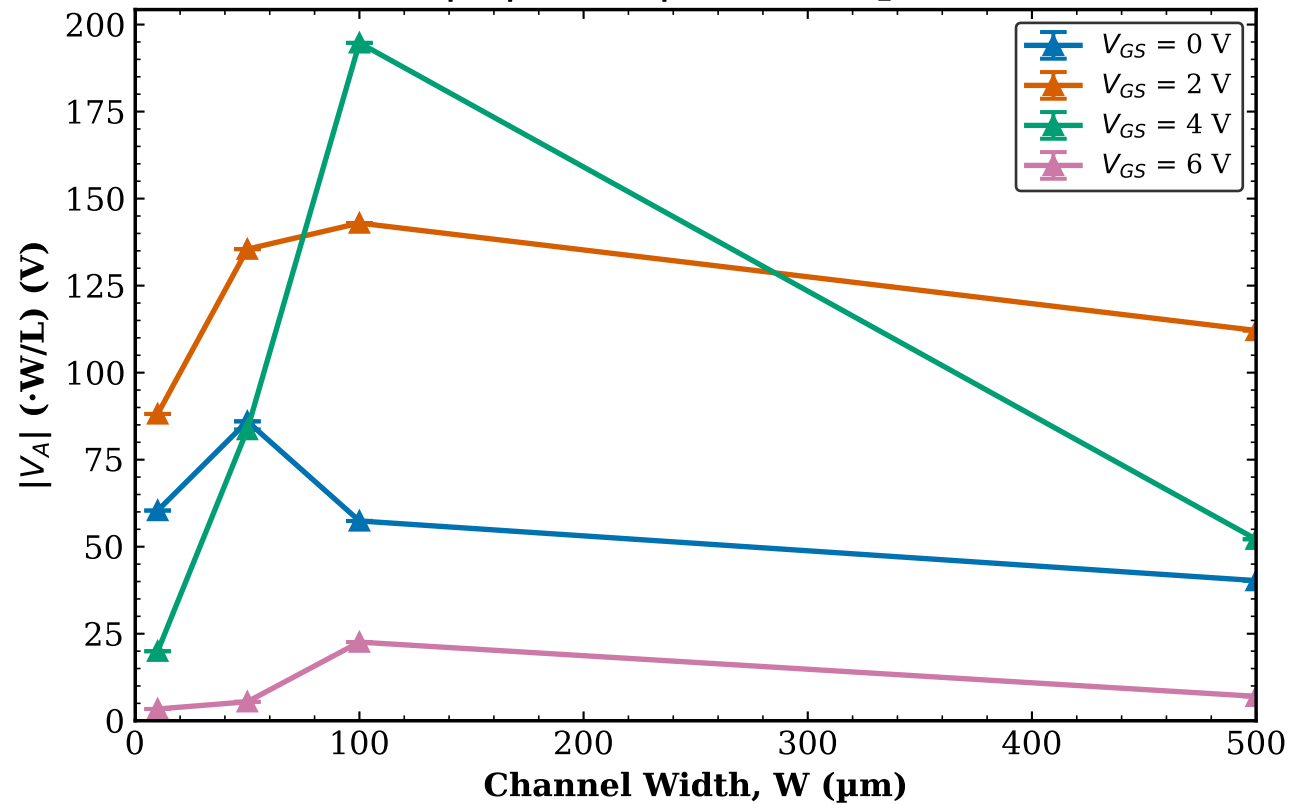
TFT2 Transistor 1 |V_A| vs W | L = 160\text{ }\mu\text{m}
